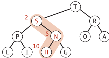
Top-down reheapify (sink)
