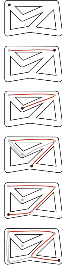
Tremaux exploration
